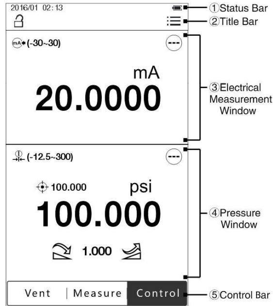
Figure 7 Main Screen
