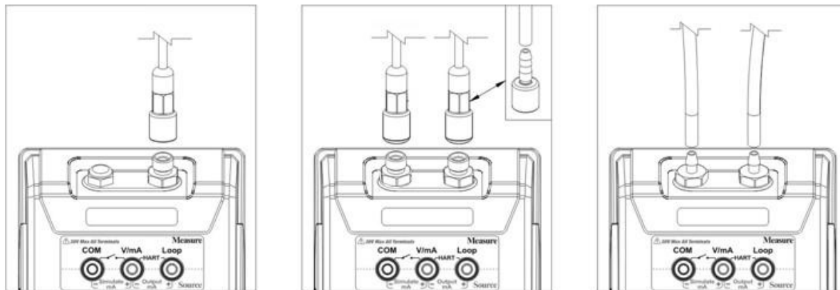
Figure 6 Pressure Connection
