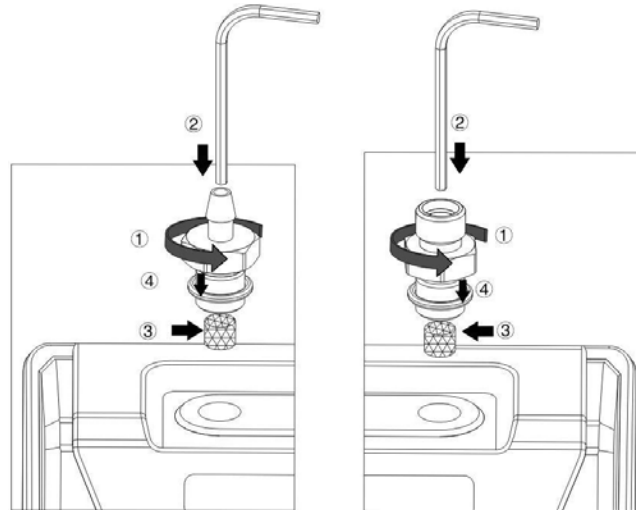
Figure 19 REF and Outlet Port Filter
