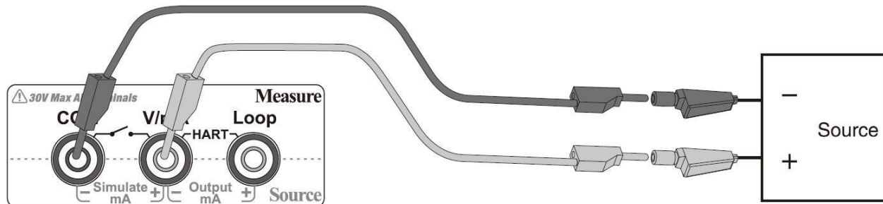
Figure 9 Current / Voltage Measurement
