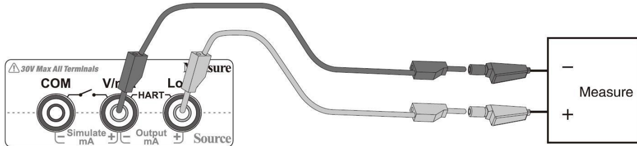
Figure 12 Current Output
