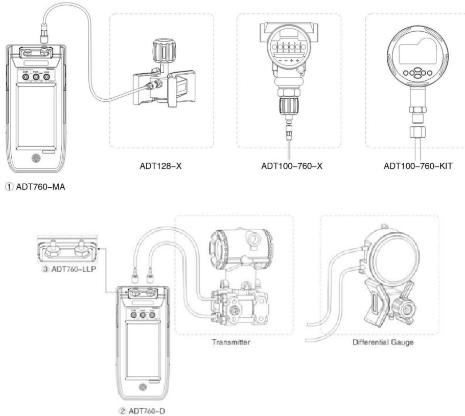
Figure 8 Output Connection
